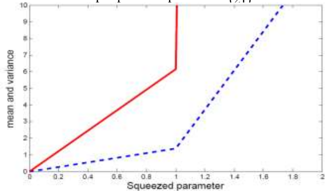
Figure 2: plots of mean (Eq. (24)) and variance of photon number(Eq.(29))
