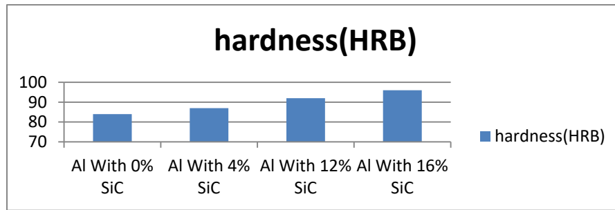
Graph between Wt % of SiC vs Hardness
