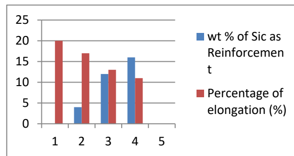
Percentage of Elongation of specimens
