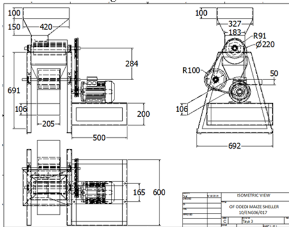
Figure 2- Isometric view of a maize sheller
